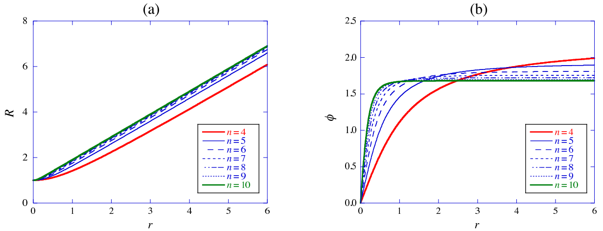
FIG. 1: The n -dimensional wormhole solutions; (a) The circumference radius R and (b) the scalar field \phi are plotted as a function of the radial coordinate r . The cases of n = 4 –10 are shown.
