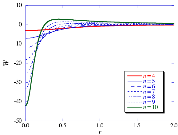
FIG. 2: The potential function W(r) is plotted. W(r) is finite everywhere, and negative around the throat.
