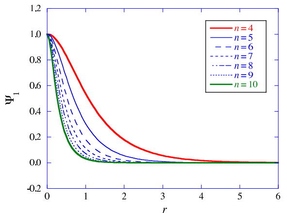
FIG. 3: The eigenfunction \Psi_1 [Eq. (3.17)] is plotted as a function of radial coordinate r .
