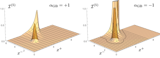
(a) large amplitude case, Gauss-Bonnet gravity
