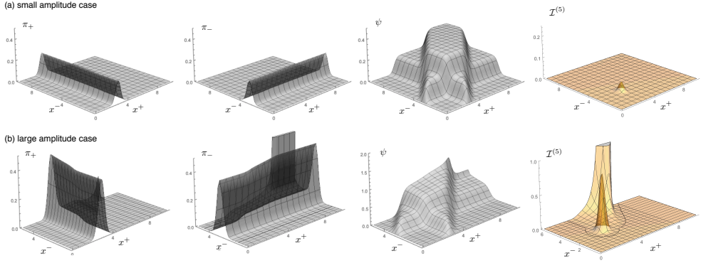
Figure 2. Evolutions of colliding two scalar pulses in five-dimensional GR: (a) the small-amplitude case [ a = 0.2 in Eqs. (8)], and (b) the large-amplitude case ( a = 0.4 ). The scalar momentum \pi_{\pm} , scalar field \psi , and the Kretschmann scalar \mathcal{I}^{(5)} are plotted in the (x^+, x^-) coordinates. Initial data were set at both \Sigma_- ( x^+ = 0, x^- > 0 ) and \Sigma_+ ( x^+ > 0, x^- = 0 ) and evolved. For small pulses, we see that they just cross, and space-time turns back toward flat again, while for large pulses, we see that nonlinear curvature evolution appears after the collision of pulses. The latter behavior is similar to the exact solutions of the plane-wave collision.
