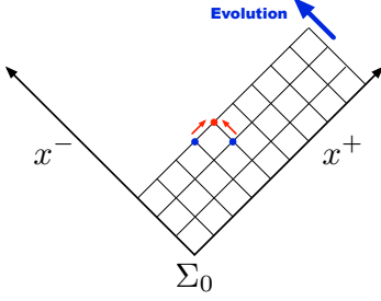
Figure 1. Numerical grid structure. Initial data are given on null hypersurfaces \Sigma_{\pm} ( x^{\mp} = 0 , x^{\pm} > 0 ) and their intersection \Sigma_0 . Generally, the initial data have to be given as (\Omega, f, \vartheta_{\pm}, \psi) on \Sigma_0 , and (v_{\pm}, \pi_{\pm}) on \Sigma_{\pm} . We then evolve the data u = (\Omega, \vartheta_{\pm}, f, v_{\pm}, \psi, \pi_{\pm}) on a constant- x^- slice to the next.
