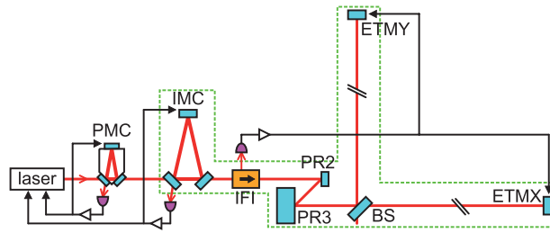
Fig. 11. Interferometer configuration of iKAGRA.
